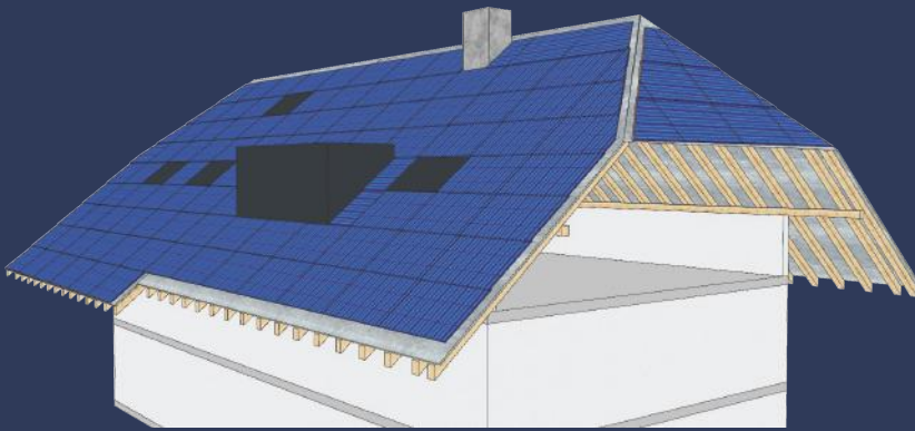
3D-Modell Solardach
